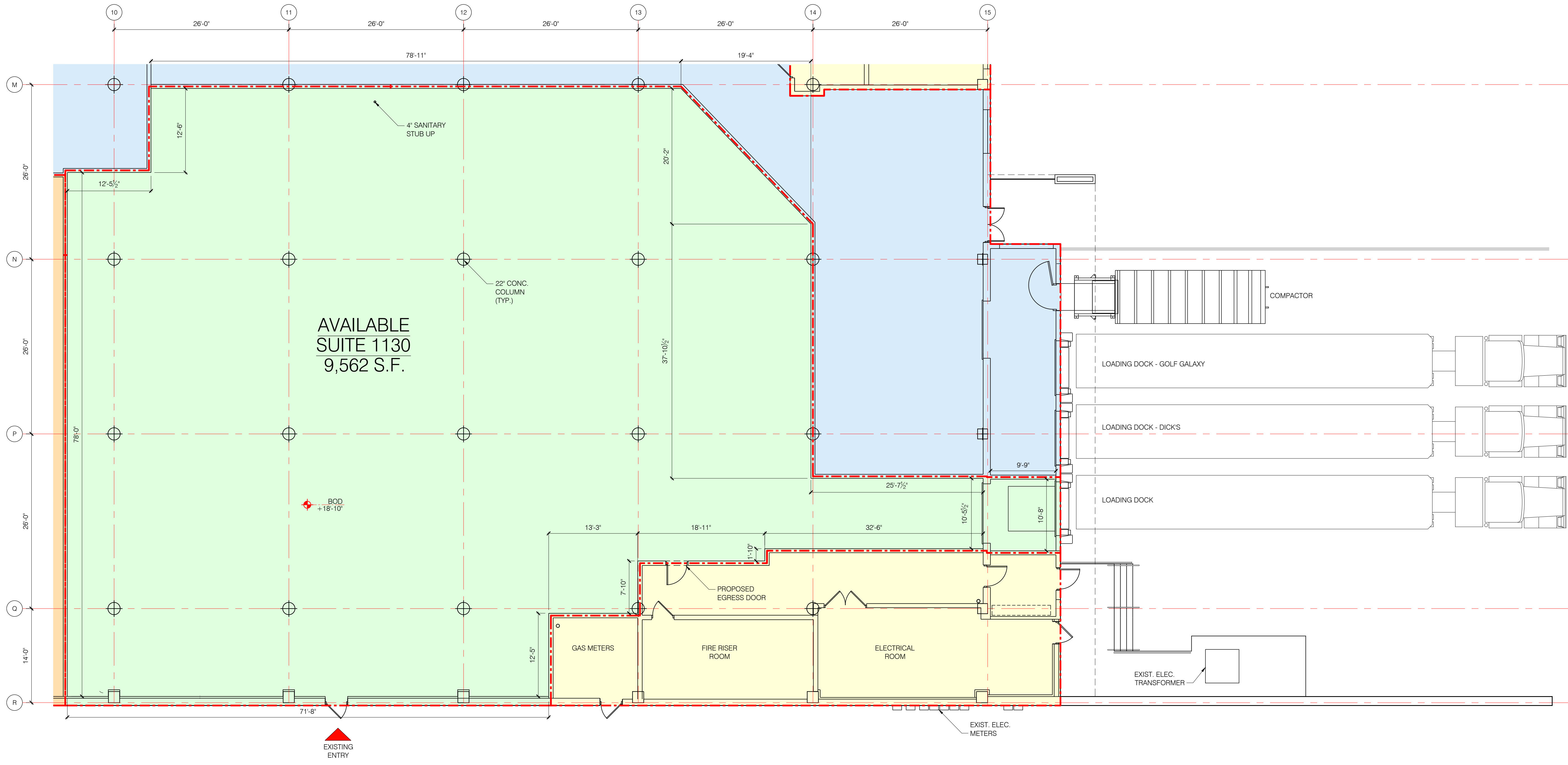
UNIT 1130 1 LOD-2 GROUND FLOOR PLAN SCALE: 1/8" = 1'-0"
